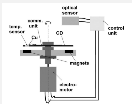
Cross-sectional schematic view of a heater "lab-on-a-disc"
